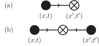
FIG. 1. Feynman diagrammatic representation of (a) the heat kernel propagator \langle u(x, t) p(x', t') \rangle_0 and (b) the velocity-velocity correlator \langle u(x, t) u(x', t') \rangle_0 .
