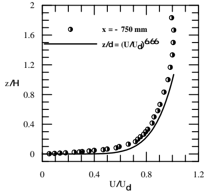
Figure 4. Longitudinal mean velocity profile, undisturbed profile.
