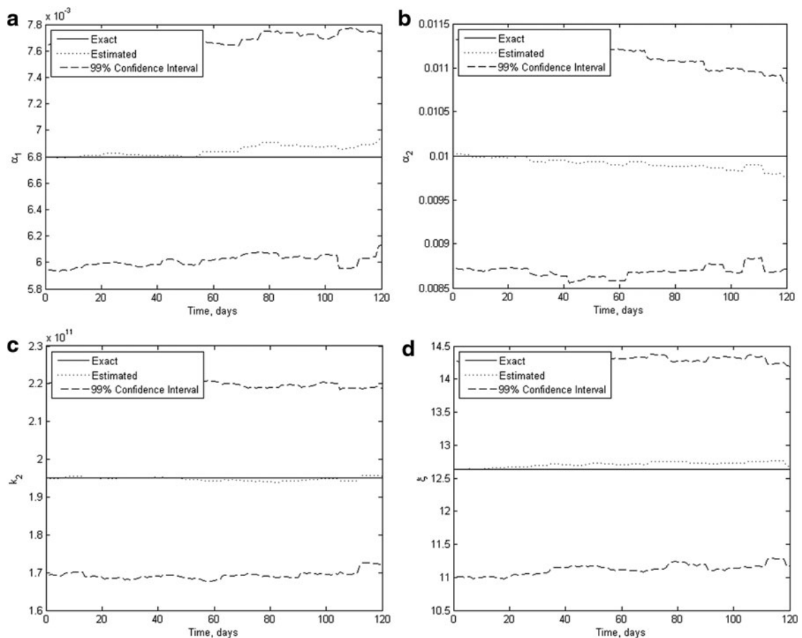
FIG. 4. Estimation of selected model parameters with 2000 particles and standard deviations of 5% for the state evolution model, measurements, and model parameters.
