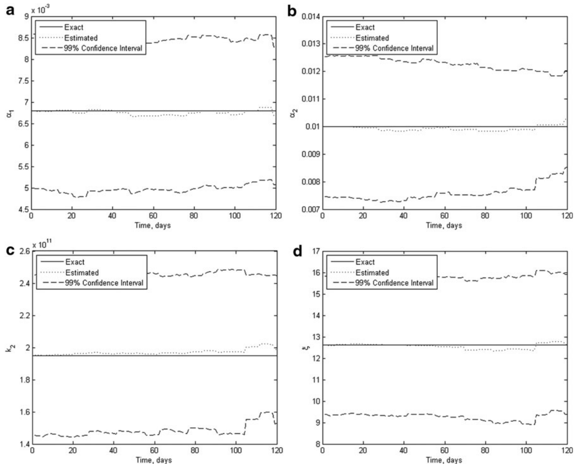
FIG. 6. Estimation of selected model parameters with 2000 particles and standard deviations of 10% for the state evolution model, measurements, and model parameters.
