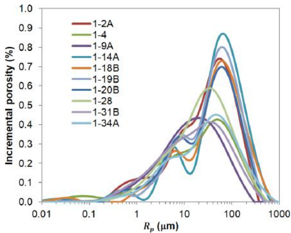
Figure 5 – NMR pore radii distribution in micrometers.
