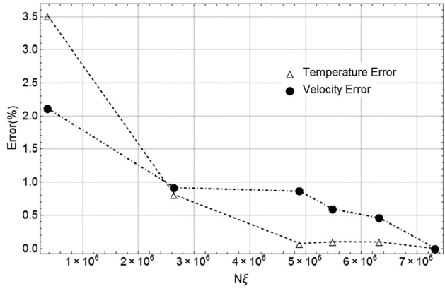
Fig. 16 Error reduction in both average velocity and top surface temperature with the increase on the total number of elements ( N\xi ) in the computational grid
