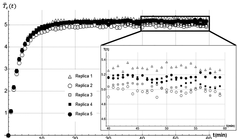
Fig. 11 Dimensionless temperature at the micro heat exchanger lower surface, at the contact with the copper cartridge, for five repeated tests at the flow rate of 20 g/min (case 1)
