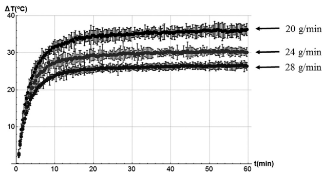
Fig. 12 Difference between the outlet (tp2) and inlet (tp1) water temperatures obtained from the thermocouple measurements, i.e., \Delta T = tp2 - tp1
